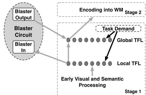
Figure 2: Revised ST 2 model implementing the two phase strength sensitivity hypothesis. The second stage, binding types to tokens using a binding pool, is not depicted, but is inherited unchanged from the basic ST 2 model (Bowman & Wyble, 2007). Links shown between individual pairs of units are replicated in one-to-one fashion across layers.
